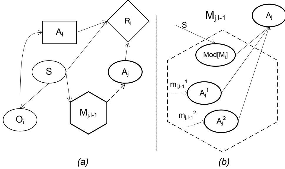
Figure 2.3: (a) Level l > 0 I-ID for agent i sharing the environment with one other agent j . The hexagon is the model node ( M_{j,l-1} ) and the dashed arrow is the policy link. (b) Representing the model node and policy link using chance nodes and causal relationships. The decision nodes of the lower-level I-IDs or IDs ( m_{j,l-1}^1, m_{j,l-1}^2 ) are mapped to the corresponding chance nodes ( A_j^1, A_j^2 ), which is indicated by the dotted arrows. Depending on the value of node, Mod[M_j] , distribution of each of the chance nodes is assigned to node A_j with some probability.
