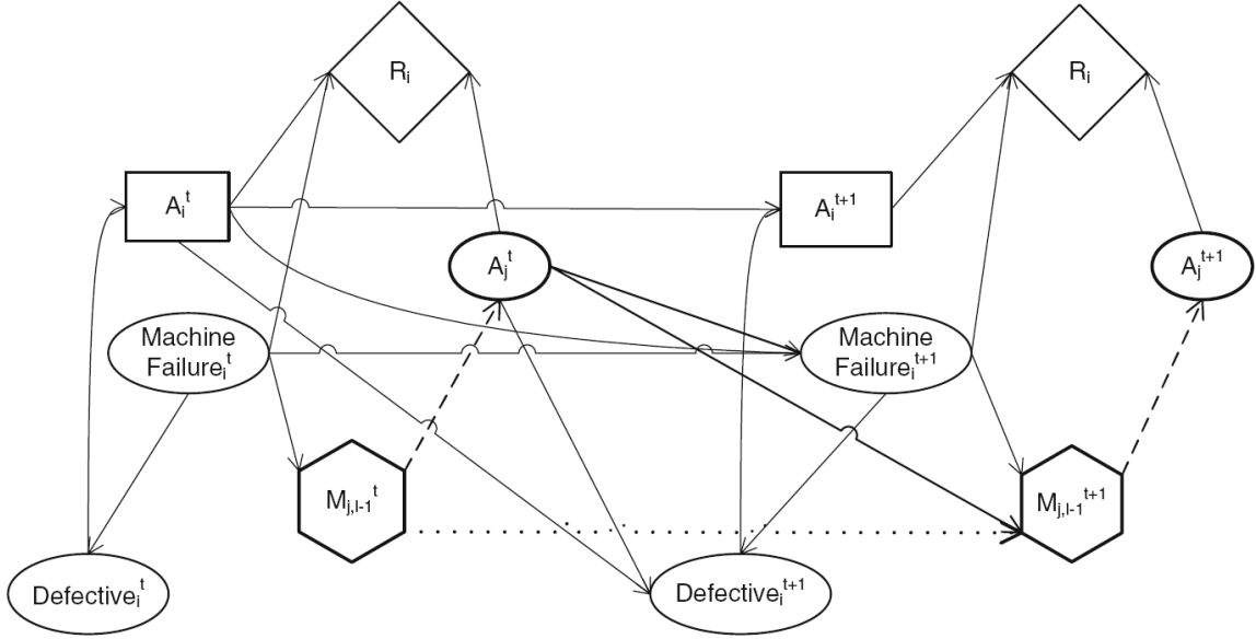
Figure 6.6: Level 1 I-DID of agent i for the multiagent MM problem. The hexagonal model node contains M level 0 DID nodes of agent j . At horizon 1, the models of j are IDs [14].
