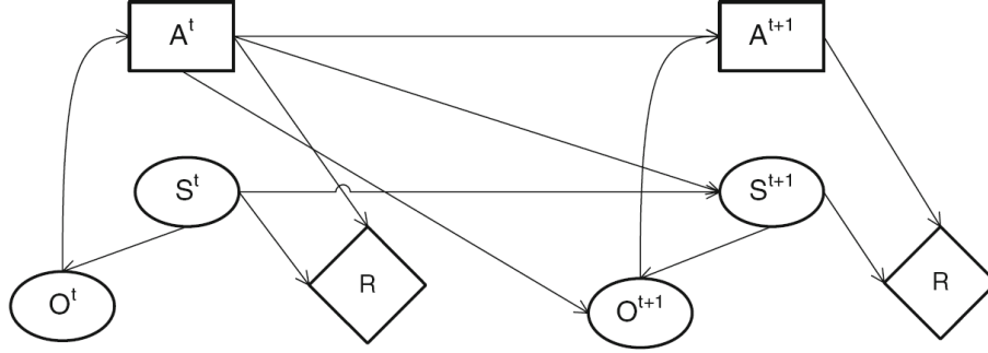
Figure 2.2: A two time-slice/horizon dynamic influence diagram (DID) representing the decision-making problem of an agent. Here, the influences (links) connect nodes not only within the same time slice but nodes across time slices as well.
