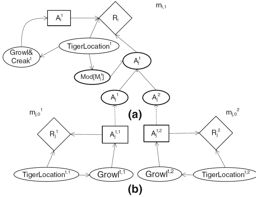
Figure 6.1: (a) Level 1 I-ID of agent i , (b) two level 0 IDs of agent j whose decision nodes are mapped to the chance nodes, A_{j,0}^1 and A_{j,0}^2 , in (a), indicated by the dotted arrows. The two IDs differ in the distribution over the chance node, TigerLocation [14].
