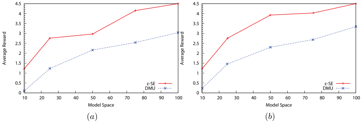
Figure 7.2: Comparison of \epsilon -SE and DMU for the multi-agent tiger problem in terms of the rewards obtained given identical numbers of models in the initial model node (a) before clustering and pruning and (b) after clustering and pruning.
