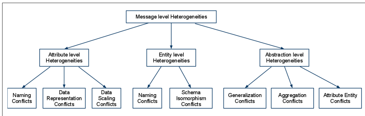
Figure 2.3: Classification of message-level heterogeneities by Nagarajan et al. [36]
