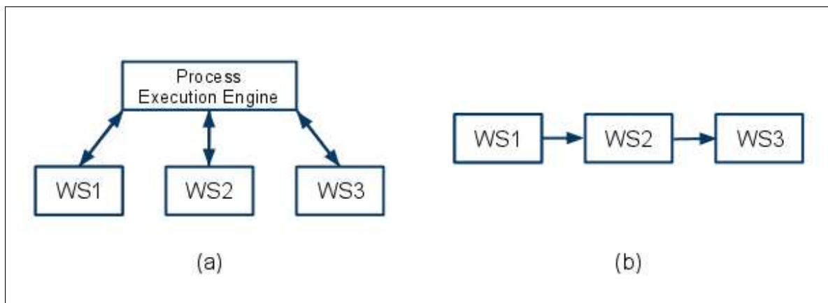
Figure 2.1: Service Composition a) Orchestration, where a central coordinator provides a controlled environment b) Choreography, where the functionality is delivered through a collaborative effort of individual Web services. Both types of service composition might require data mediation
