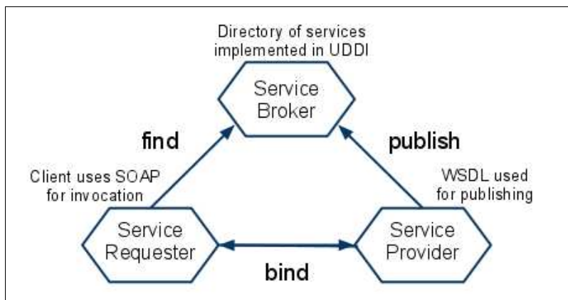
Figure 1.1: The SOA model composed of Web service provider, Web service consumer and the service broker
