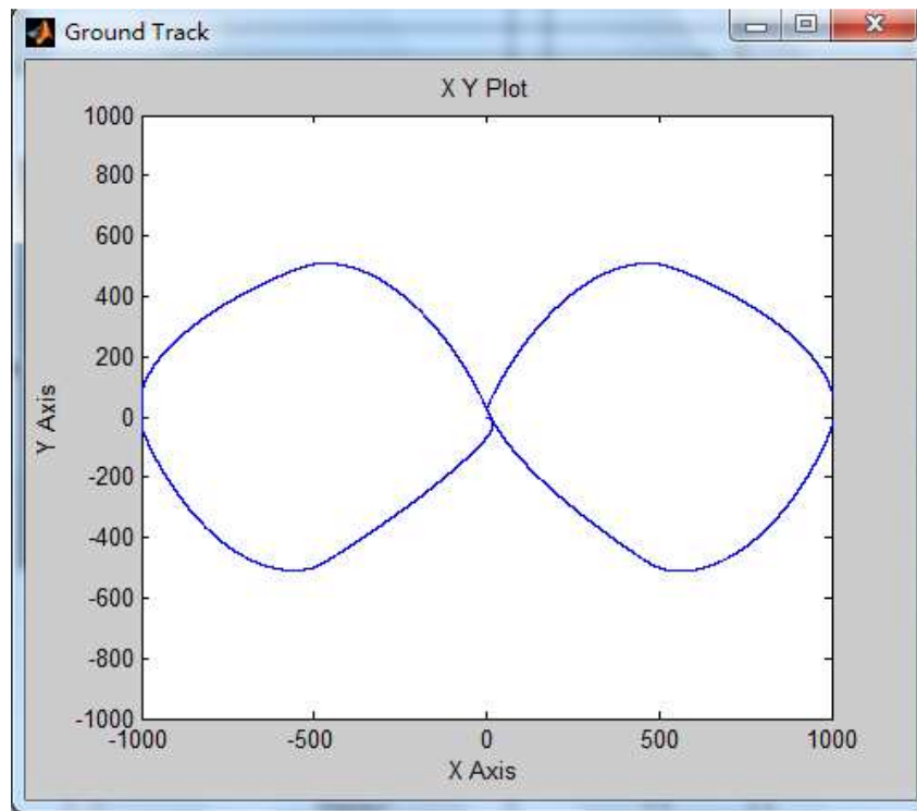
Figure 25. Ground track of a successful completion of figure eight flight pattern
