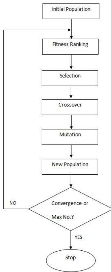
Figure 1. Flow Chart for a Genetic Algorithm
