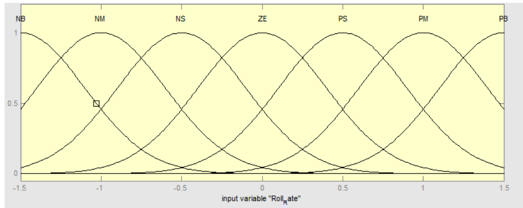
Figure 15. An evenly distributed membership function for roll rate 2
