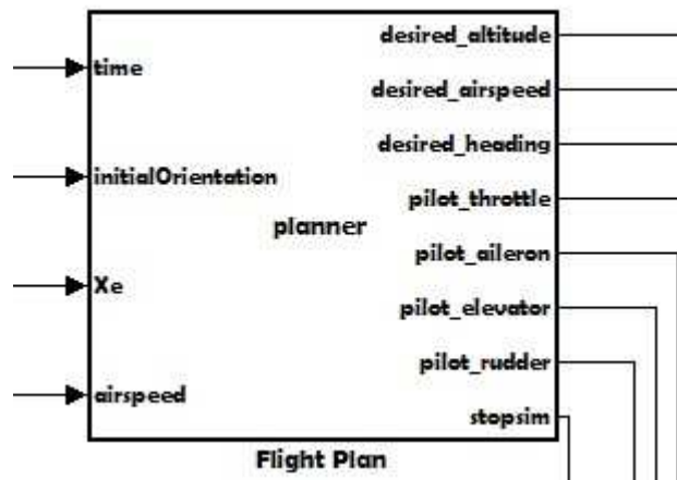
Figure 11. The Flight planner block
