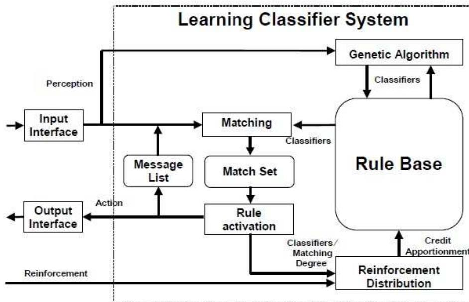
Figure 4. A generic architecture of a Learning Classifier System
