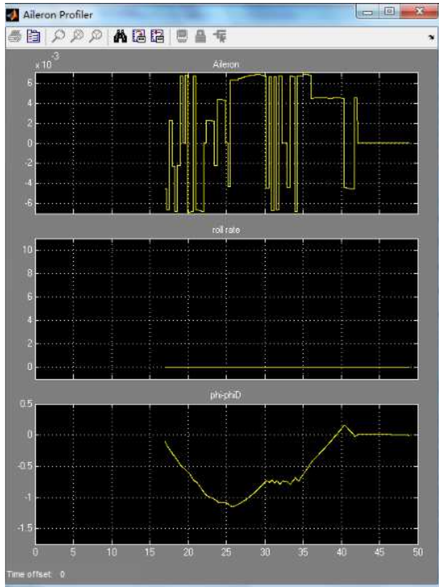
Figure 20. Initial trials in lateral control
