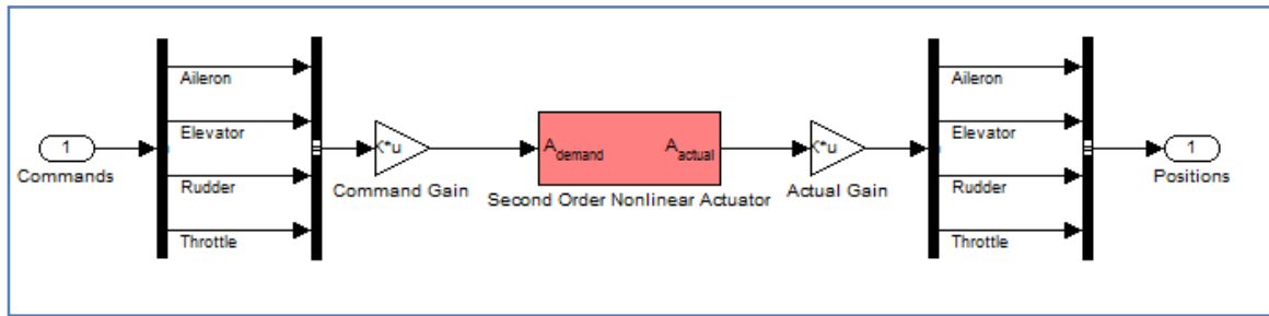
Figure 8. The Actuators block
