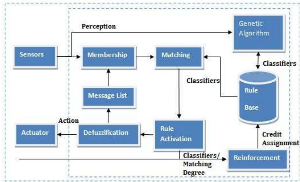
Figure 13. The UAV Learning Fuzzy Classifier System Controller Architecture
