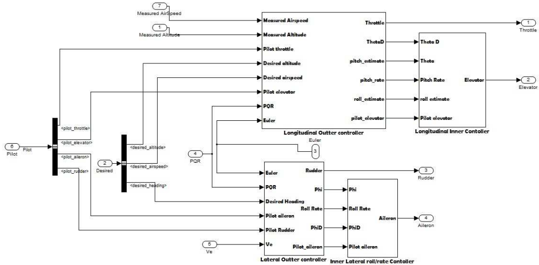
Figure 10. The Controller Model
