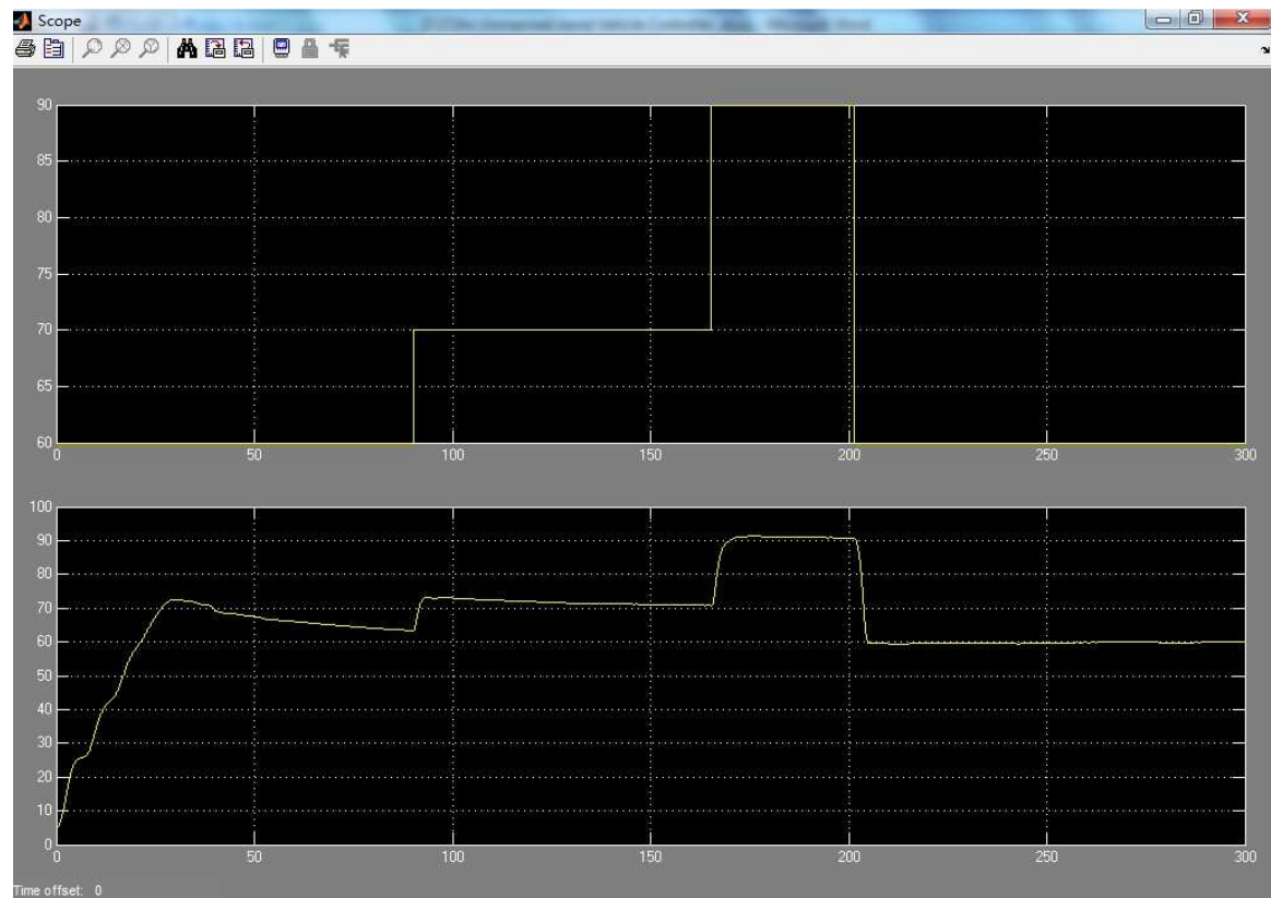
Figure 26. Altitude change of a successful completion of a figure eight flight pattern
