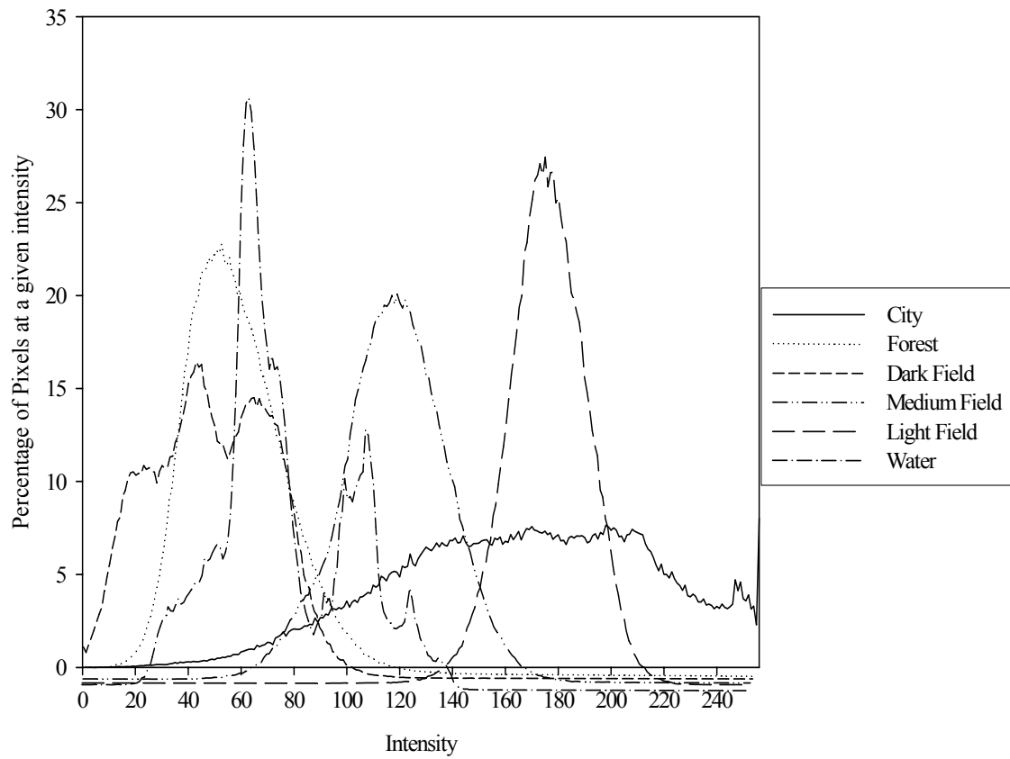
Fig. 1.2. Normalized histogram of intensities for each class.
