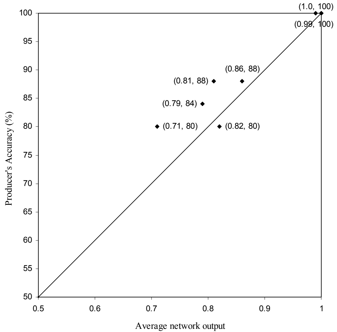
Fig. 3.1. Average network output for the seven classes on the evaluation data set versus Producer's accuracy for textural approach (coordinates of each point are in paranthesis).
