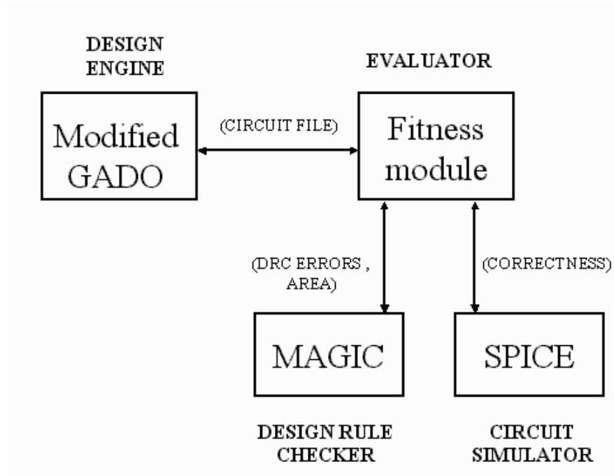
Figure 4.2: Architecture
