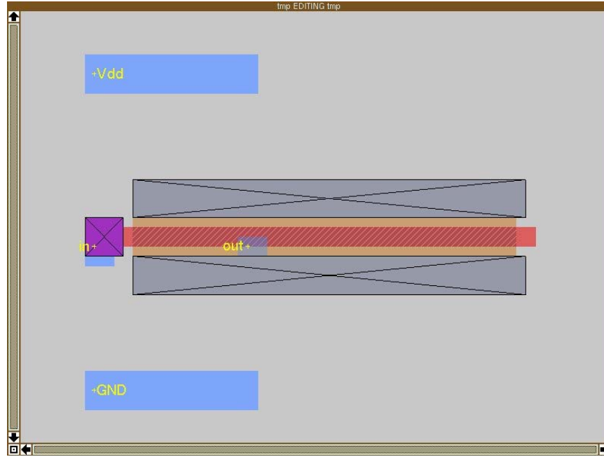
Figure 3.1: Current attempt at an Inverter.
