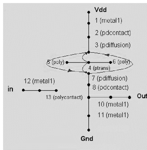
Figure 4.8: Connectivity Graph corresponding to cell in Figure 4.7
