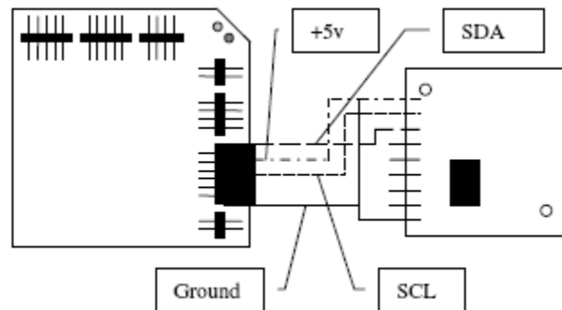
Figure 3.2 The Brainstem/CMPS03 Interface
