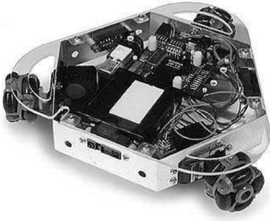
Figure 2.1 The Acroname Brainstem PPRK
