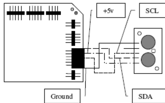
Figure 3.1 The Brainstem/SRF08 Interface
