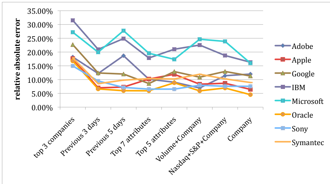
Fig 1:- This figure shows relative absolute error for predicting the highest price for eight companies using neural network. The second dataset is used as testing set in this case
