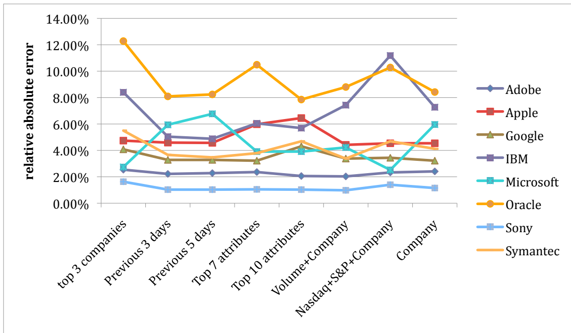
Fig 8:- This figure shows relative absolute error for predicting highest price for eight companies using MSP. The third dataset is used as testing set in this case
