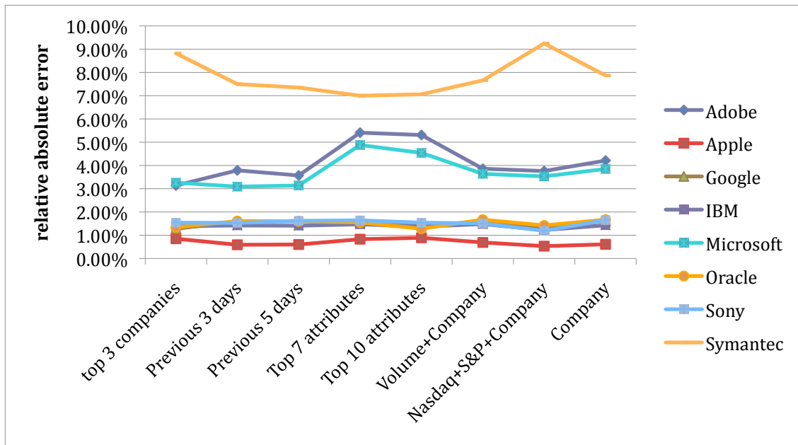
Fig 5:- This figure shows relative absolute error for predicting highest price for eight companies using bagging approach. The second dataset is used as testing set in this case.
