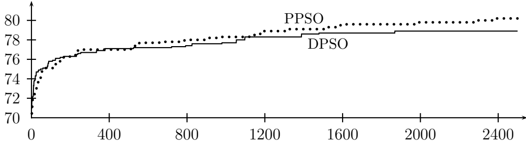
Figure 5.1: Comparison of mean adjusted fitness for SIB
