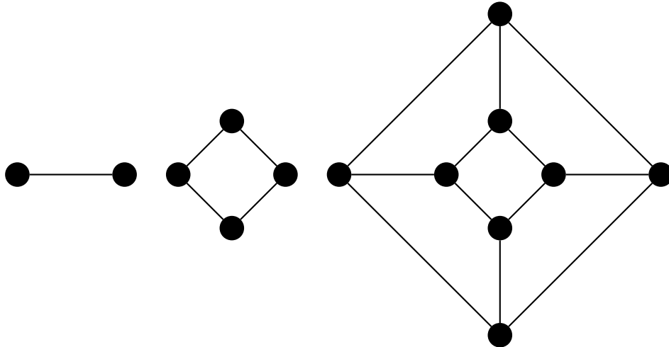
Figure 4.4: Hypercubes in dimensions 1–3
