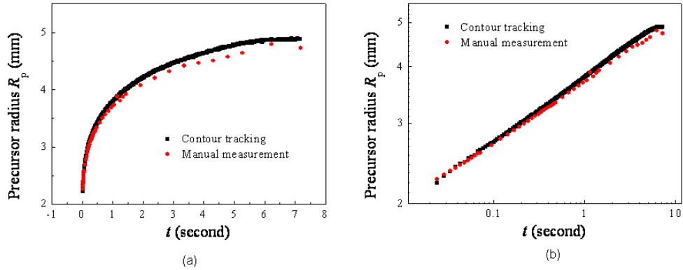
Figure 5.1: Comparison of the evolution of the precursor radius R_p over time t calculated from manual measurement and using the Contour Tracker on a (a) linear scale and (b) log-log scale.
