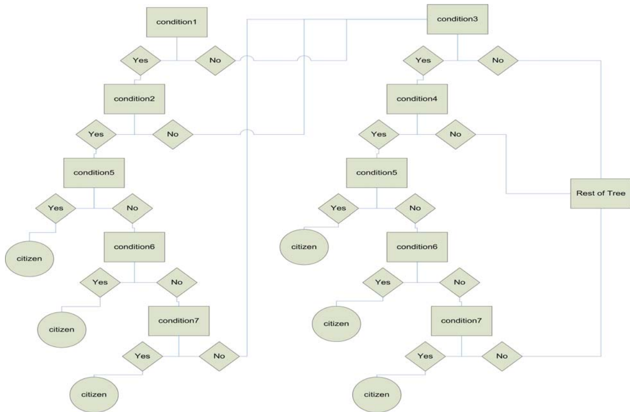
Figure 3.2: THE RULES FROM FIGURE 3.1 AS THEY WOULD APPEAR IN A DECISION-TREE REPRESENTATION
