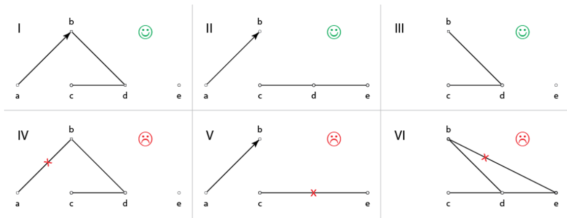
Figure 6: Sample subgraphs. I, II, and III are valid subgraphs of the sample graph in Figure 1. IV, V, and VI are invalid subgraphs of same. An 'x' indicates the violations in each invalid subgraph.
