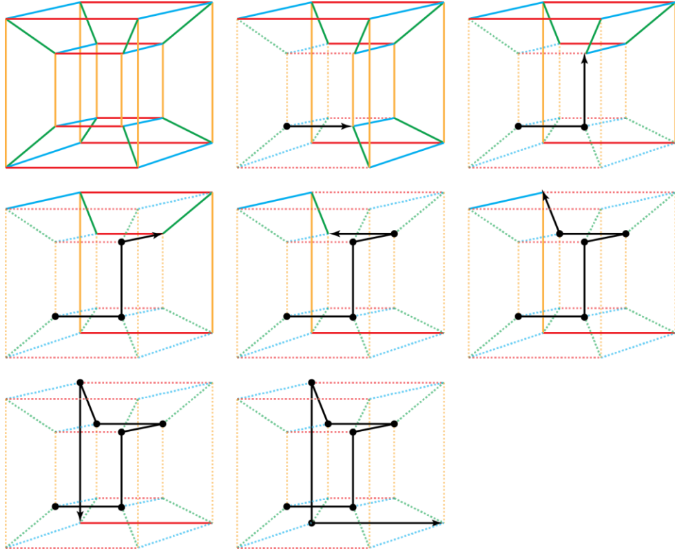
Figure 10: The number of available nodes shrinks rapidly as the path builds. 4-cube example. Parallel edges are colored alike. Solid edges are available for transition. Dotted edges are unavailable.
