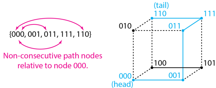
Figure 8: Sample induced path as an ordered set (left) and in the 3-cube graph (right). In the 3-cube, the dashed edges here indicate chords connecting to non-path nodes.) In an induced path all non-consecutive path nodes are \geq 2 distant.
