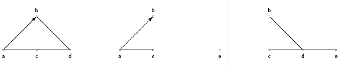
Figure 7: Sample induced subgraphs. These three subgraphs are valid induced subgraphs of the sample graph in Figure 1.
