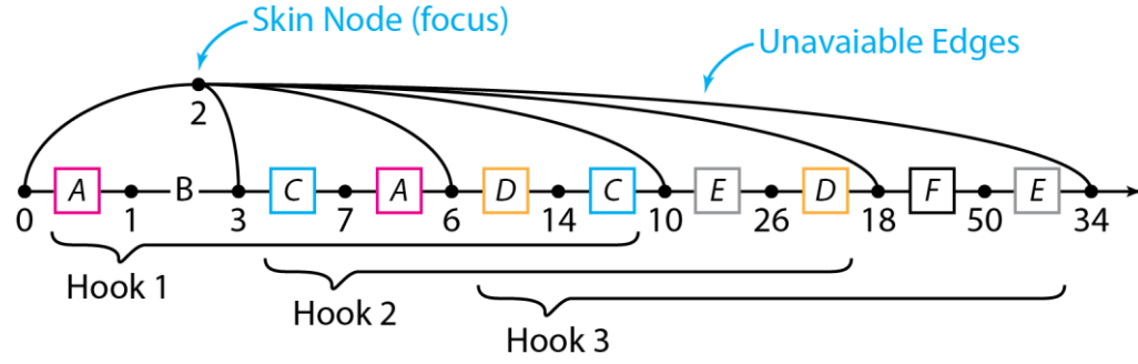
Figure 11: Snake of hooks orbiting a single skin node. Here nodes of an ( n \geq 6 )-cube are laid out in a line. Only nodes and edges specific to the example are pictured. Solid dots are nodes and are correctly numbered. Solid lines are edges. Letter symbols indicate a chain of hooked ladder patterns. The TS correlating to the numbered nodes is 0 1 2 0 3 2 4 3 5 4 ...
