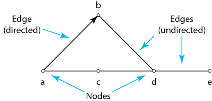
Figure 1: A sample graph with nodes and edges indicated.
