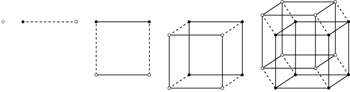
Figure 2: Hypercube graphs for 0 \leq n \leq 4 (left to right respectively). Solid nodes joined by solid edges show previous n -cube in current n -cube. Hollow nodes joined by solid edges show duplication of previous n -cube in current n -cube. Dashed edges show new edges in the current n -cube.
