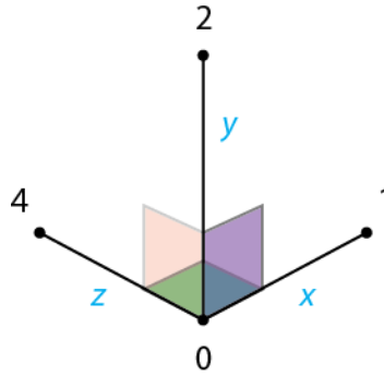
Figure 3: Example of orthogonal (mutually perpendicular) edges. z \perp y \perp x \perp \dots
