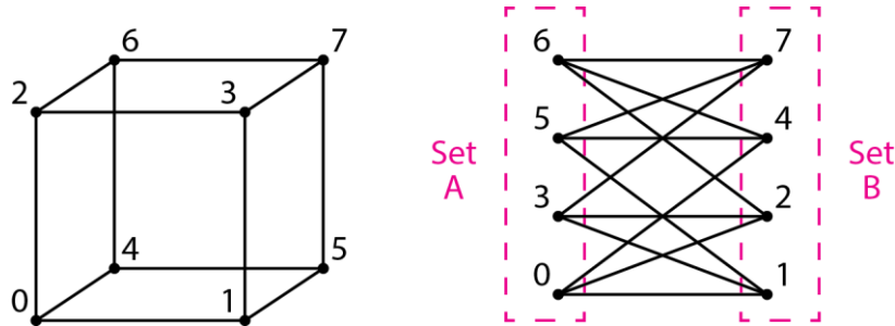
Figure 4: Hypercube graphs are regular (both), and bipartite (right).
