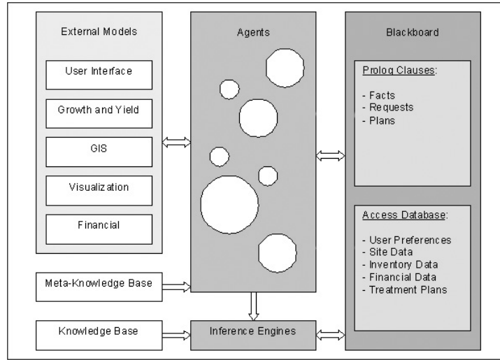
Figure 1.2: NED-2 Architecture
