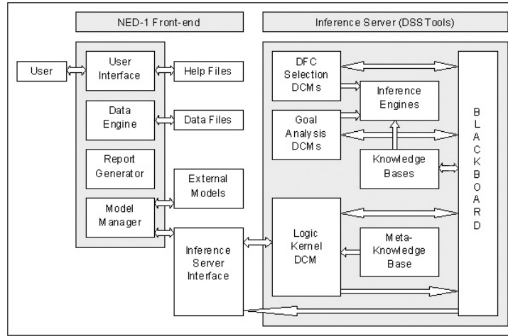
Figure 1.1: NED-1 Architecture
