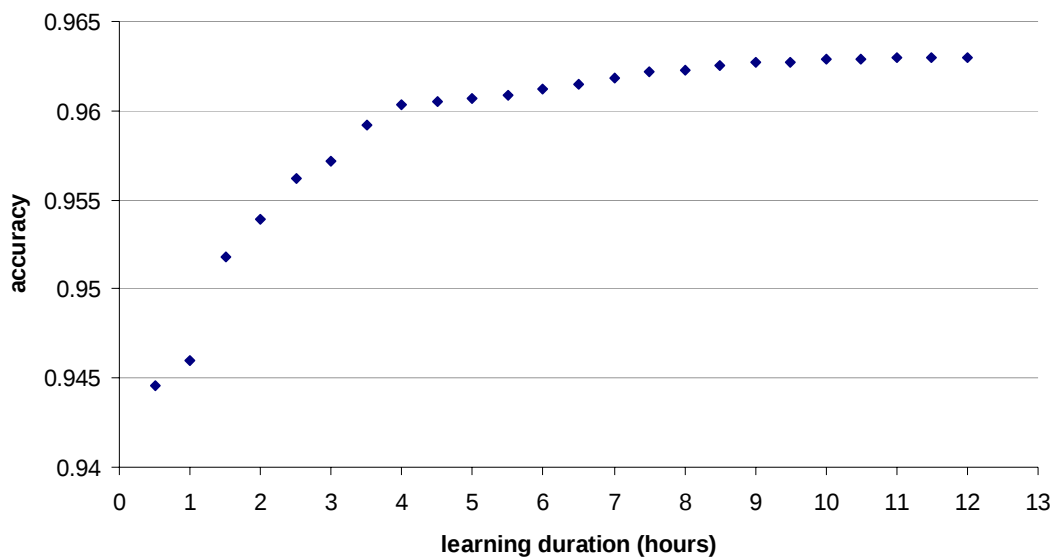
Figure 5.3 The 12 hours' learning progress
