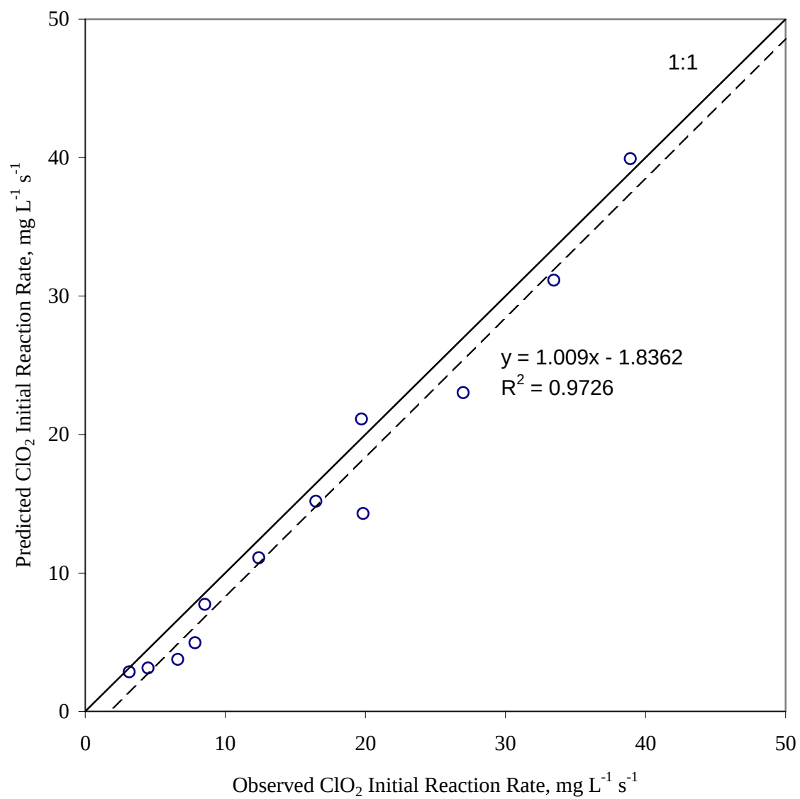
Fig. 3.4 Prediction of \text{ClO}_2 initial reaction rates with ethanethiol at \text{pH}=3.73
