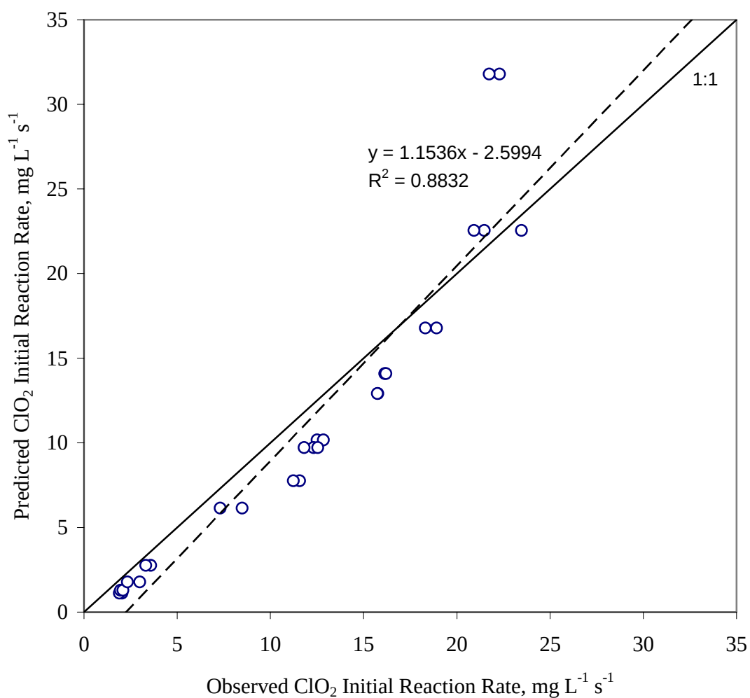
Fig. 3.10 Prediction of \text{ClO}_2 initial reaction rates with DMDS at pH = 6.92
