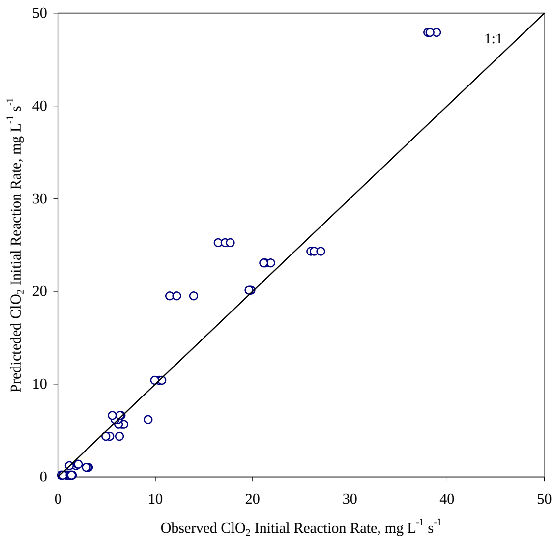
Fig. 4.4 Prediction of \text{ClO}_2 initial reaction rates with ethanethiol and DMDS mixtures, randomly partitioning data.
