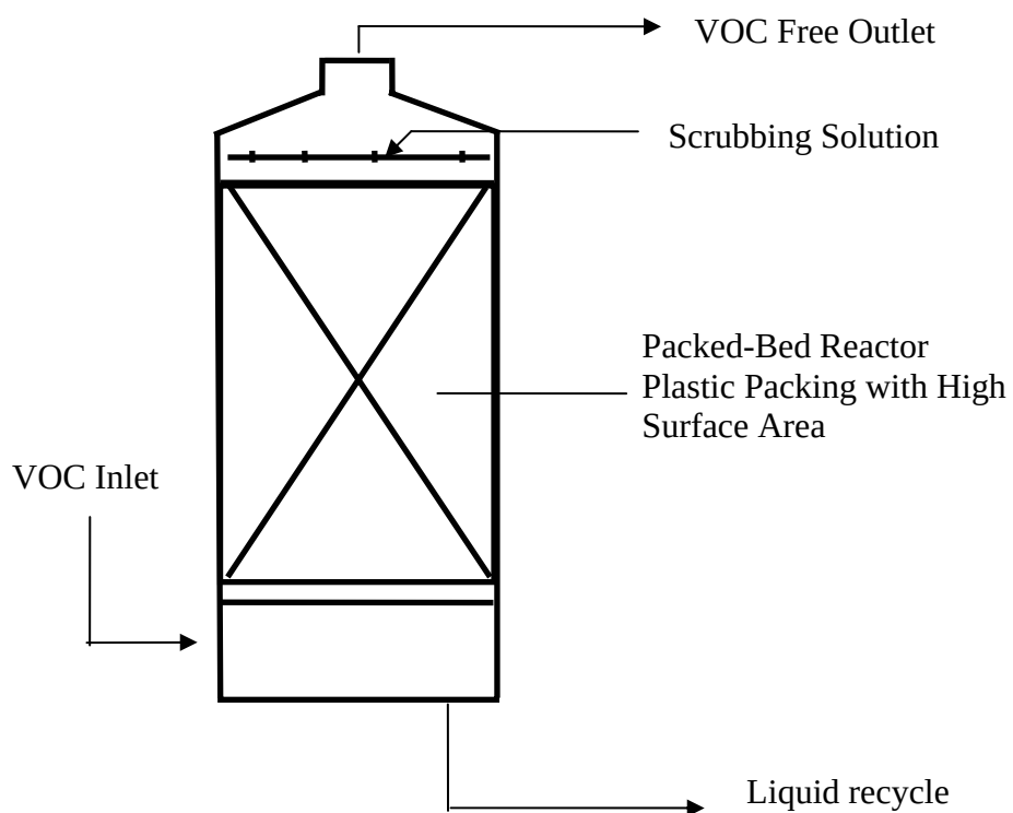
Fig. 3.1 Wet scrubber system
