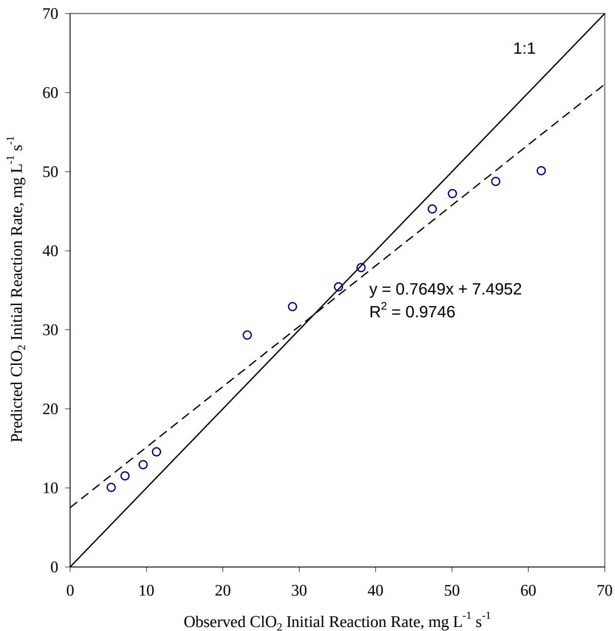
Fig. 3.6 Prediction of \text{ClO}_2 initial reaction rates with ethanethiol at pH=4.01
