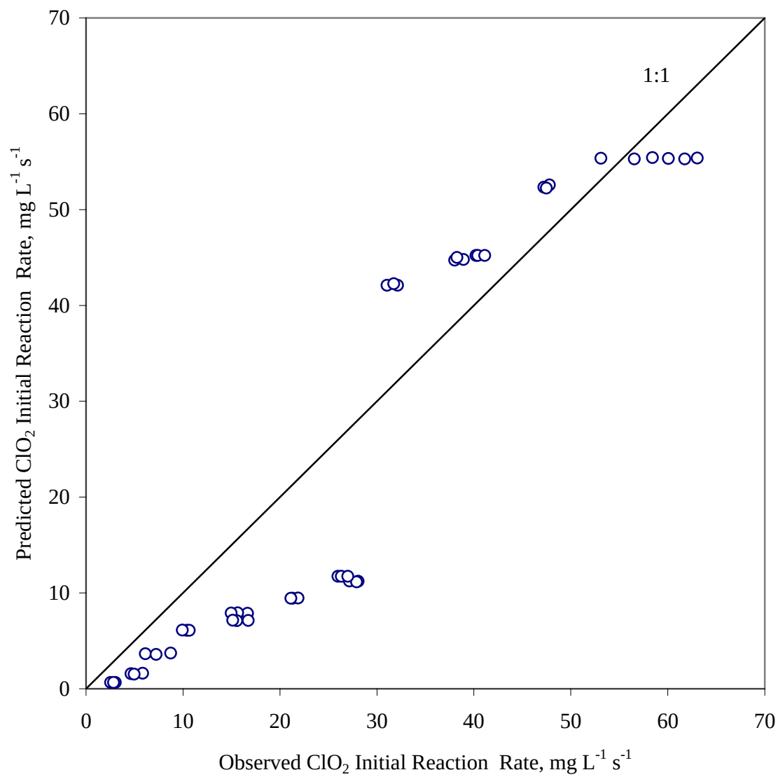
Fig. 4.3 Prediction of \text{ClO}_2 initial reaction rates with ethanethiol and DMDS mixtures at pH = 5.80
