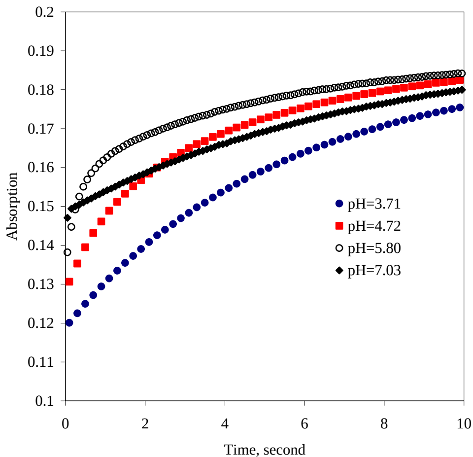
Fig. A.2 Absorption changes at 250 nm in the reaction of 60 mg/L \text{ClO}_2 with 10 mg/L ethanethiol and 10 mg/L DMDS mixtures at 30°C and different pH levels
