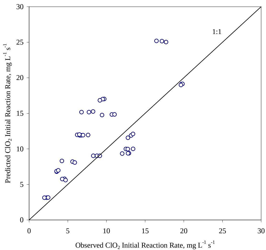
Fig. 4.2 Prediction of \text{ClO}_2 initial reaction rates with ethanethiol and DMDS mixtures at \text{pH}=4.72
