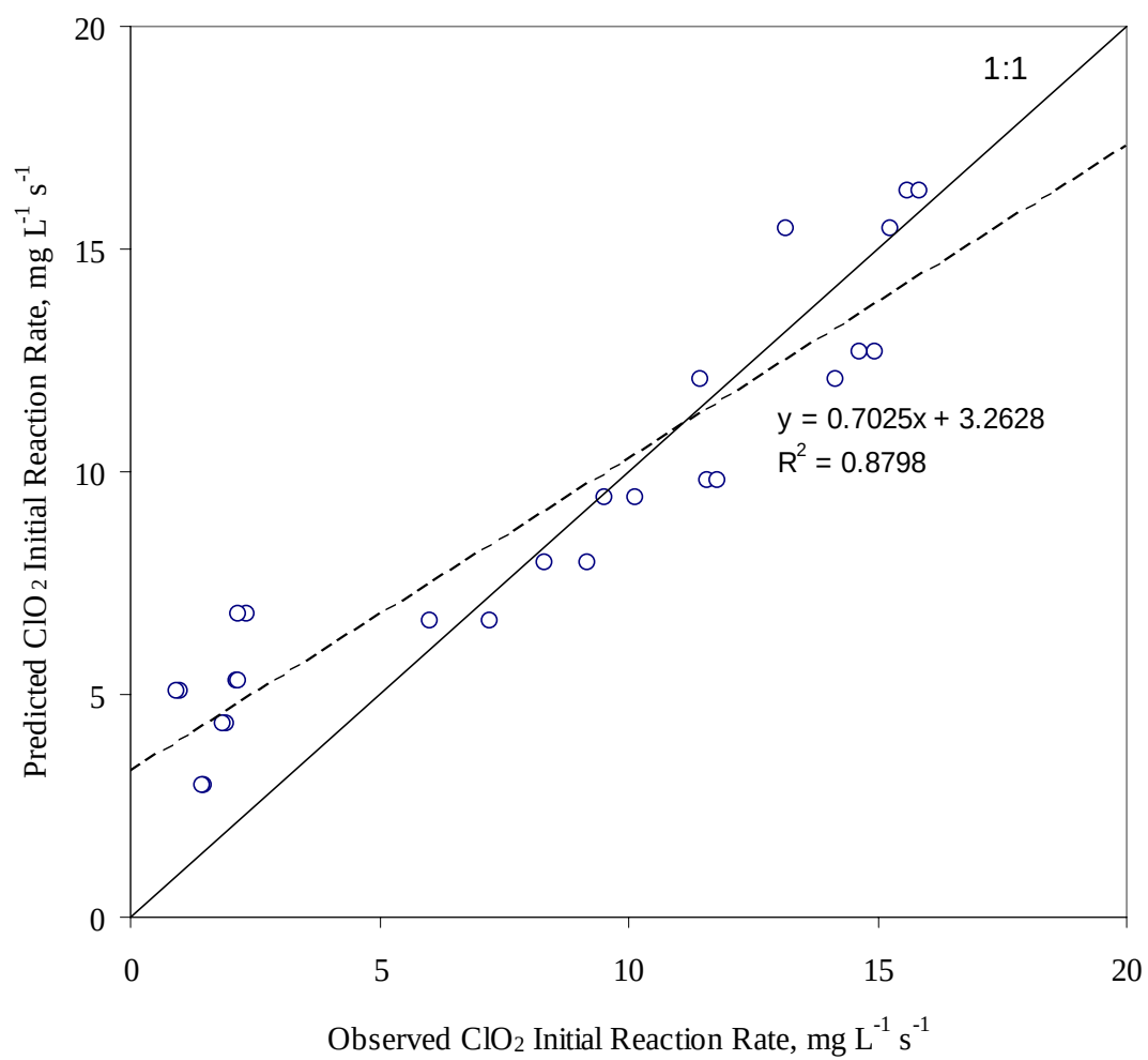
Fig. 3.12 Prediction of \text{ClO}_2 initial reaction rates with DMDS at pH = 9.02
