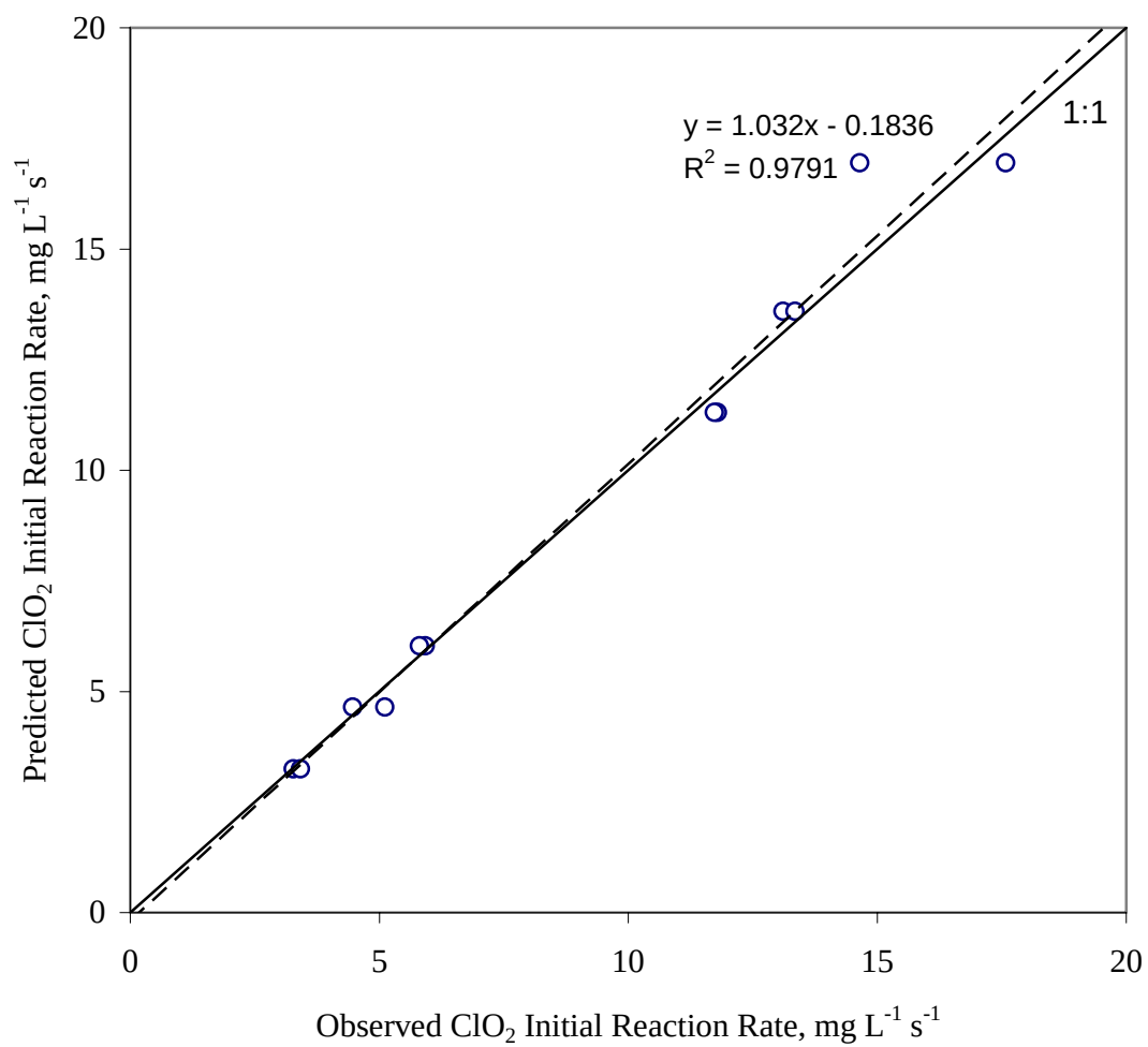
Fig. 3.9 Prediction of \text{ClO}_2 initial reaction rates with DMDS at pH = 5.26
