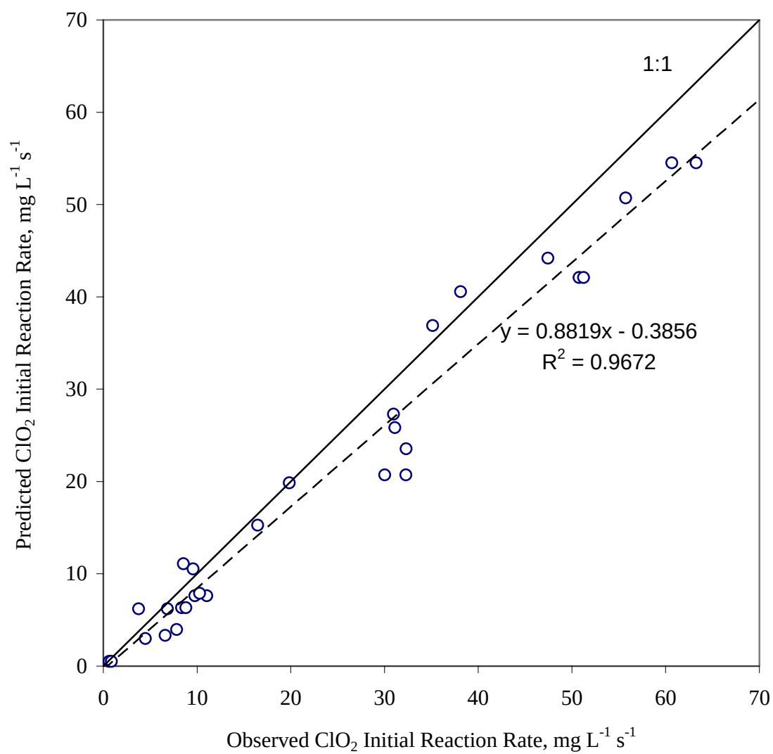
Fig. 3.7 Prediction of \text{ClO}_2 initial reaction rates with ethanethiol, general model
