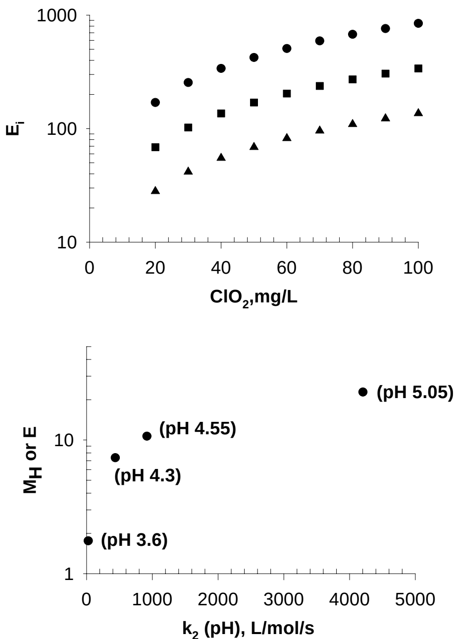
Figure 2.6 The effect of \text{ClO}_2 concentration (A) at three different inlet methanethiol concentrations, 4 (●), 10 (■), and 25 (▲) ppmv on E_i and the effect of pH on the Enhancement factor, E , for methanethiol (B). All parameters in the model were calculated at a temperature of 35^\circ\text{C} and the rate constant measured for ethanethiol was assumed valid for methanethiol.
