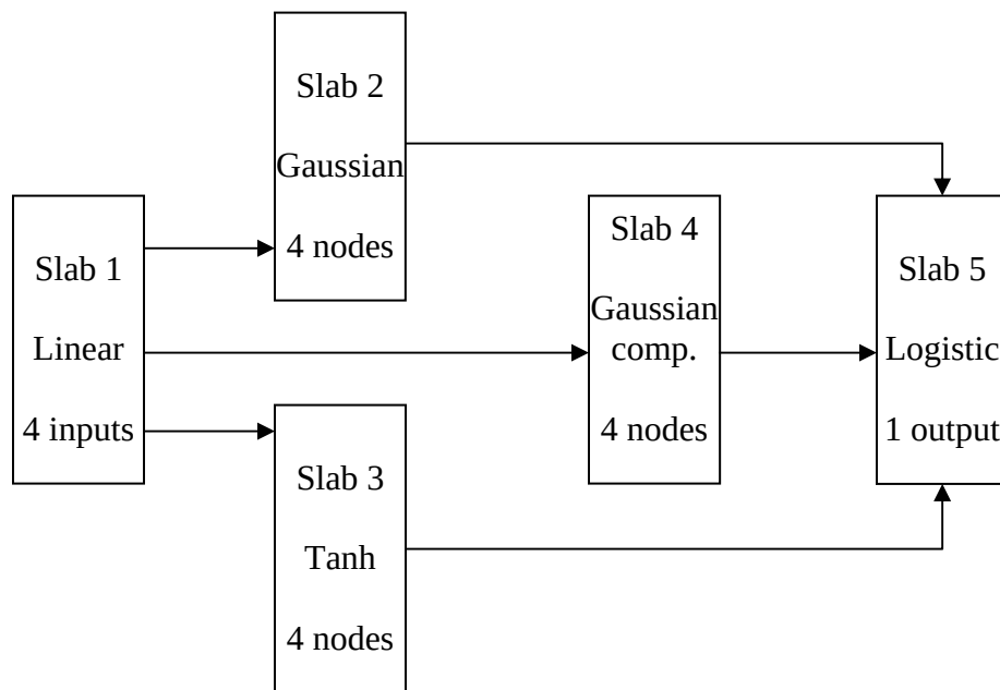
Fig. 4.1 Topology of a Ward net, activation functions, and nodes in each layer
