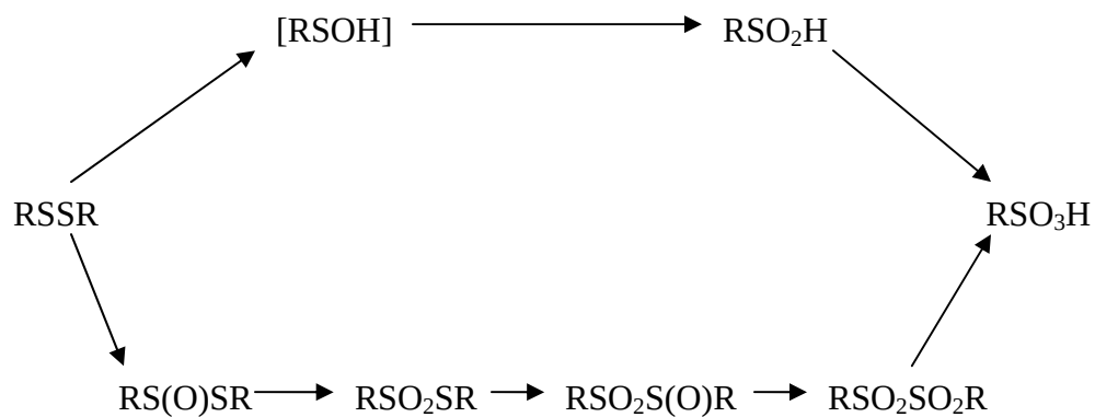
Fig. 3.2 Oxidation of disulfide (Oae, 1977)
