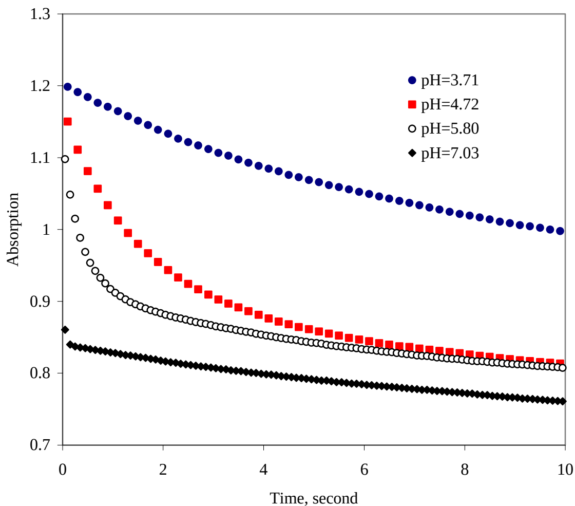
Fig. A.1 Absorption changes at 358 nm in the reaction of 60 mg/L \text{ClO}_2 with 10 mg/L ethanethiol and 10 mg/L DMDS mixtures at 30°C and different pH levels
