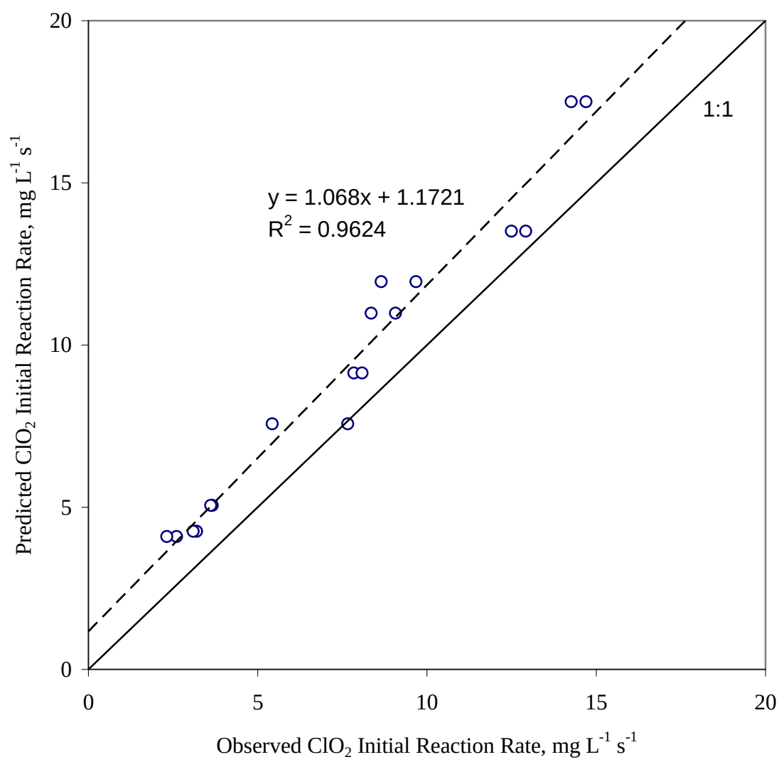
Fig. 3.11 Prediction of \text{ClO}_2 initial reaction rates with DMDS at pH = 7.62
