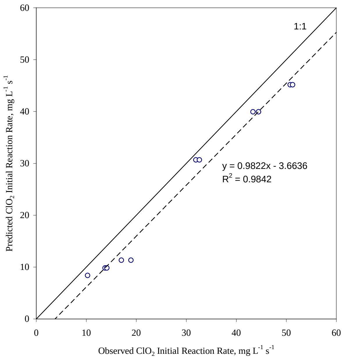
Fig. 3.5 Prediction of \text{ClO}_2 initial reaction rates with ethanethiol at pH = 3.92
