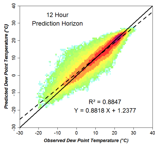
Figure 6. Predicted and observed dew point temperature, combined model, model evaluation dataset.
