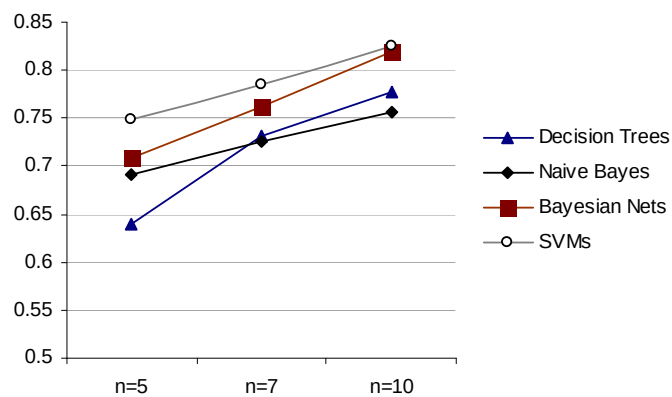
Figure 7.2: Average F1 measures over five 20-newsgroup categories at different values of n .
