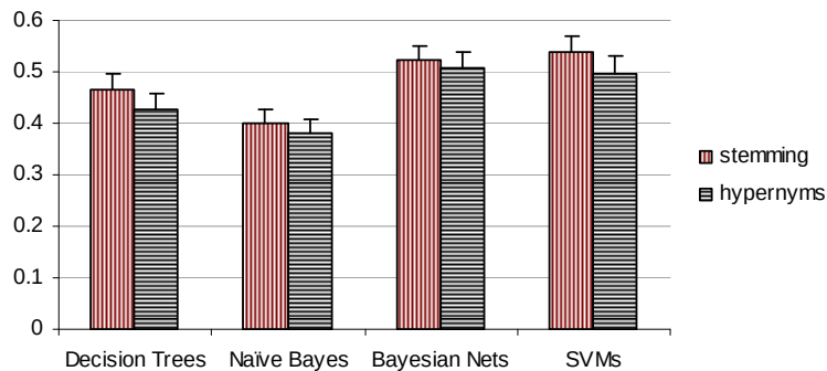
Figure 6.3: Comparison of the average F1 measures and standard errors of stemming-based representation with best performing hypernym-based representation over twenty 20-Newsgroup categories
