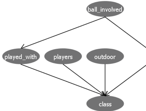
Figure 3.2: Conditional dependence/independence between the attributes of the instances in the Table 3.1.
