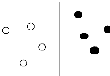
Figure 3.3: Instances in a two dimensional space separated by a line
