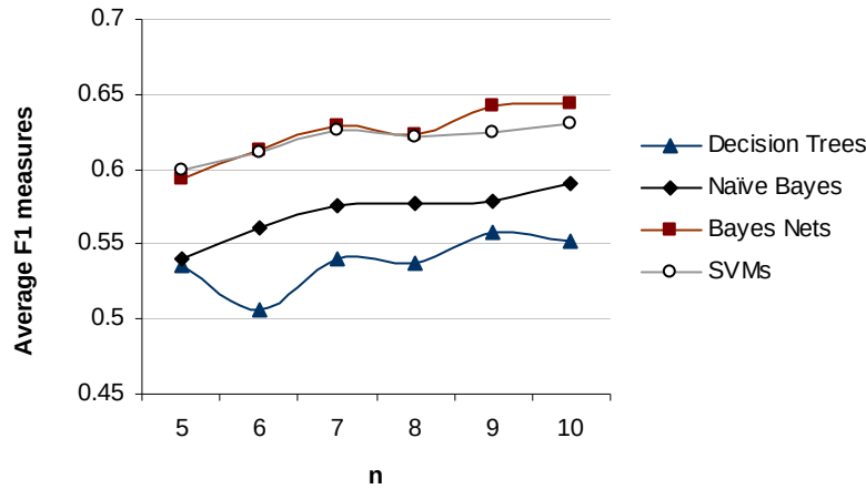
Figure 7.1: Average F1 measures over 10 frequent Reuters categories at different values of n .
