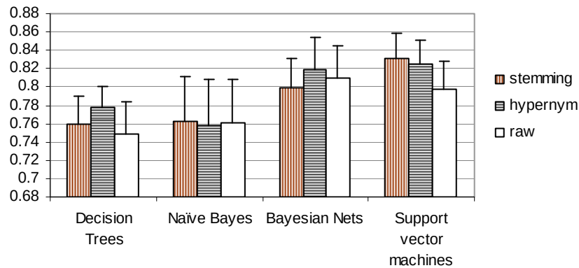
Figure 6.1: Comparison of the average F1 measures and standard errors of stemming-based representation with best performing hypernym-based representation and raw text representation
