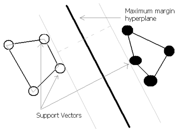
Figure 3.4: Maximum Margin Hyperplane
