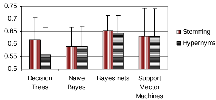
Figure 5.1: Comparison of stemming-based representation with best performing hypernym-based representation, for all four learners, in terms of average F1 measures and standard errors.
