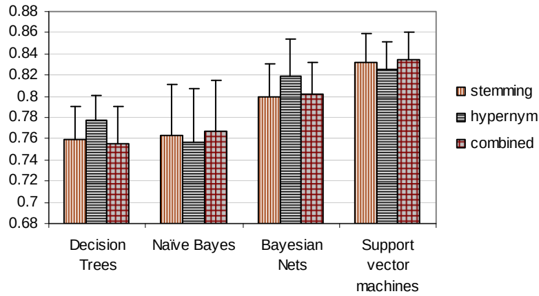
Figure 6.2: Comparison of the average F1 measures and standard errors of stemming-based representation with best performing hypernym-based and combined representations
