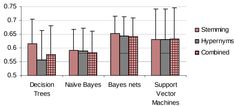
Figure 5.2: Comparison of the average F1 measures and standard errors of stemming-based representation with best performing hypernym-based and combined representations
