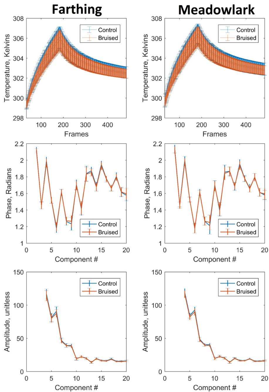
Figure 3.6. Mean thermal waveforms, mean phase values, and mean amplitude values for bruised and healthy treatment groups, separated by cultivar.
