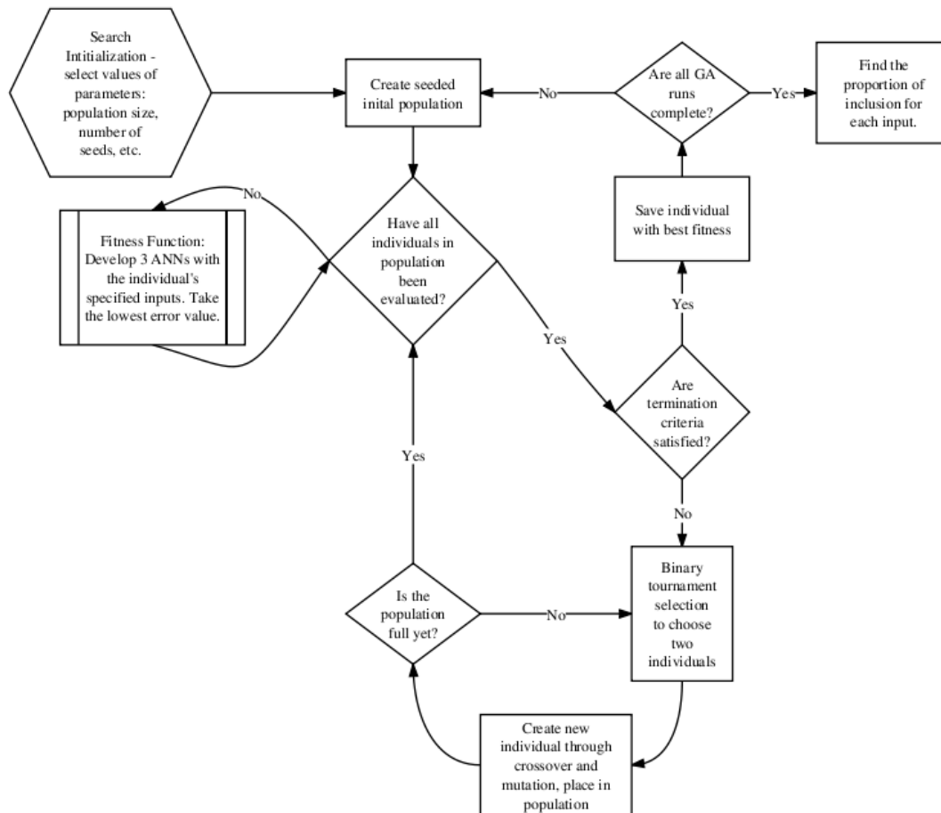
Figure 2.1 - Flowchart depicting the GA search process.
