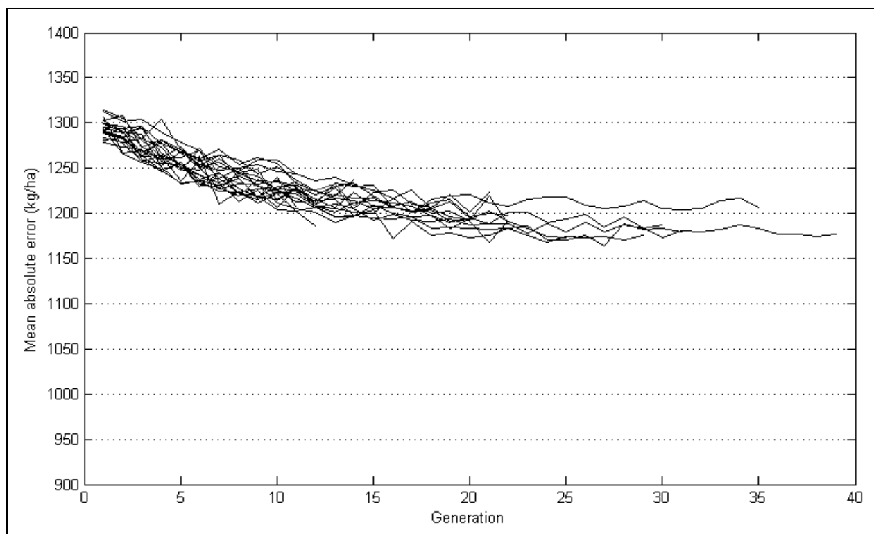
Figure 3.3: Average Mean Absolute Error on the development set for each generation of the 20 genetic algorithm runs for the January prediction date.
