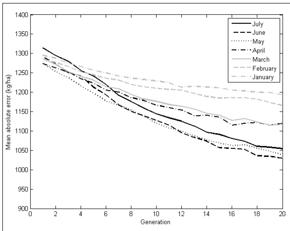
Figure 3.1: Average development set mean absolute error for seven prediction dates. Each line is averaged from 20 runs of the genetic algorithm.
