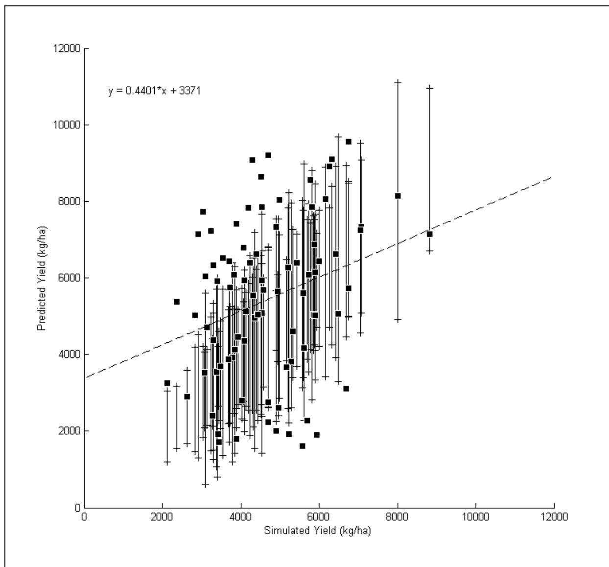
Figure 2.5 – Final ANN model yield predictions vs. target simulated yield for the evaluation data set. Error bars show \pm one standard deviation for all counties in a district for a given year, average standard deviation of 1923 kg/ha.
