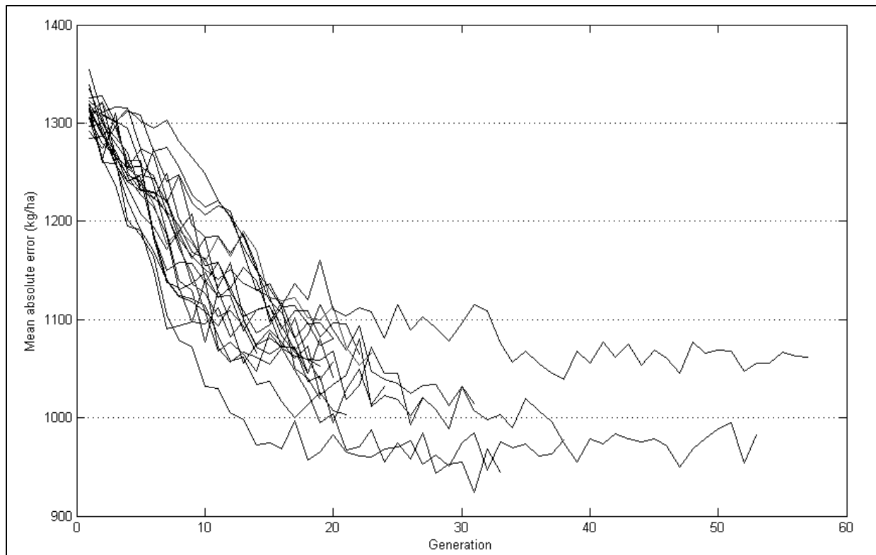
Figure 2.2 – Development set Mean Absolute Error for each generation from each of the 20 GA runs.
