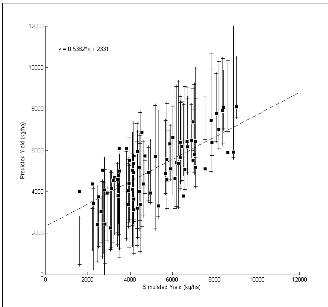
Figure 2.4 – Final ANN model yield predictions vs. target simulated yield for the selection data set. Error bars show +/- one standard deviation for all counties in a district for a given year, average standard deviation of 1920 kg/ha.
