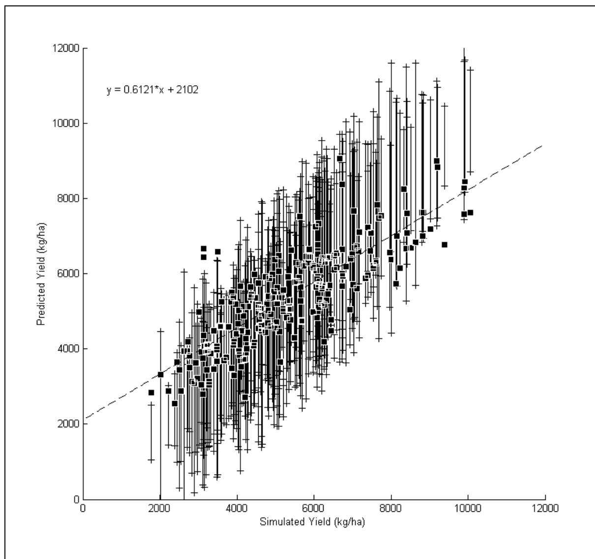
Figure 2.3 – Final ANN model yield predictions vs. target simulated yield for the development data set. Error bars show +/- one standard deviation for all counties in a district for a given year, average standard deviation of 2032 kg/ha.
