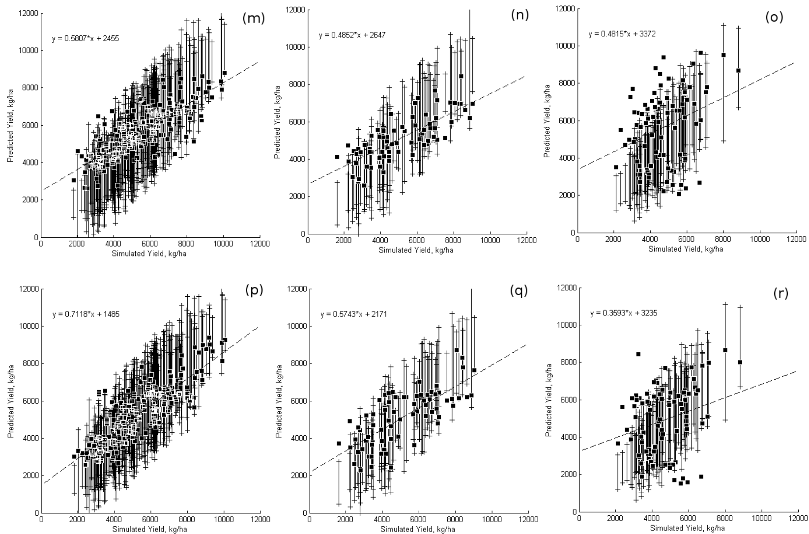
Figure 3.4 (cont.): Yield predictions vs. target simulated yield for March development (m), selection (n), and evaluation (o) sets, and for the February development (p), selection (q), and evaluation (r) sets.
