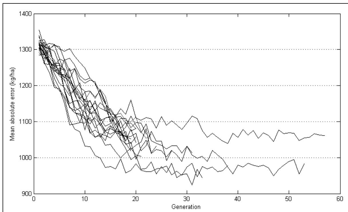
Figure 3.2: Average fitness expressed as mean absolute error on the development set for each generation of the 20 genetic algorithm runs for the July prediction date.
