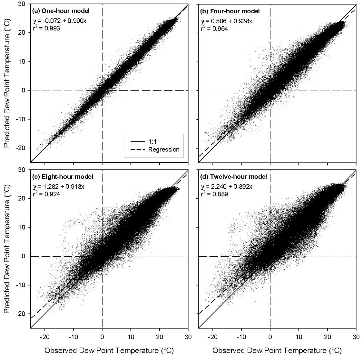
Figure 2.4: Performance of predicted dew point temperature for the evaluation dataset for the (a) one-hour, (b) four-hour, (c) eight-hour, and (d) twelve-hour prediction models
