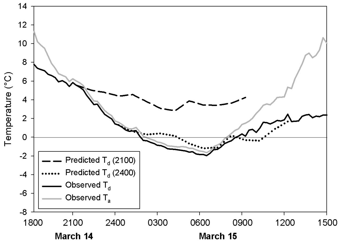
Figure 2.7: Predicted dew point temperature at 2100 and 2400 on March 14 to 15, 2005 based on a sequence of twelve models for Tiger, GA. Observed dew point temperature and air temperature are also shown.
