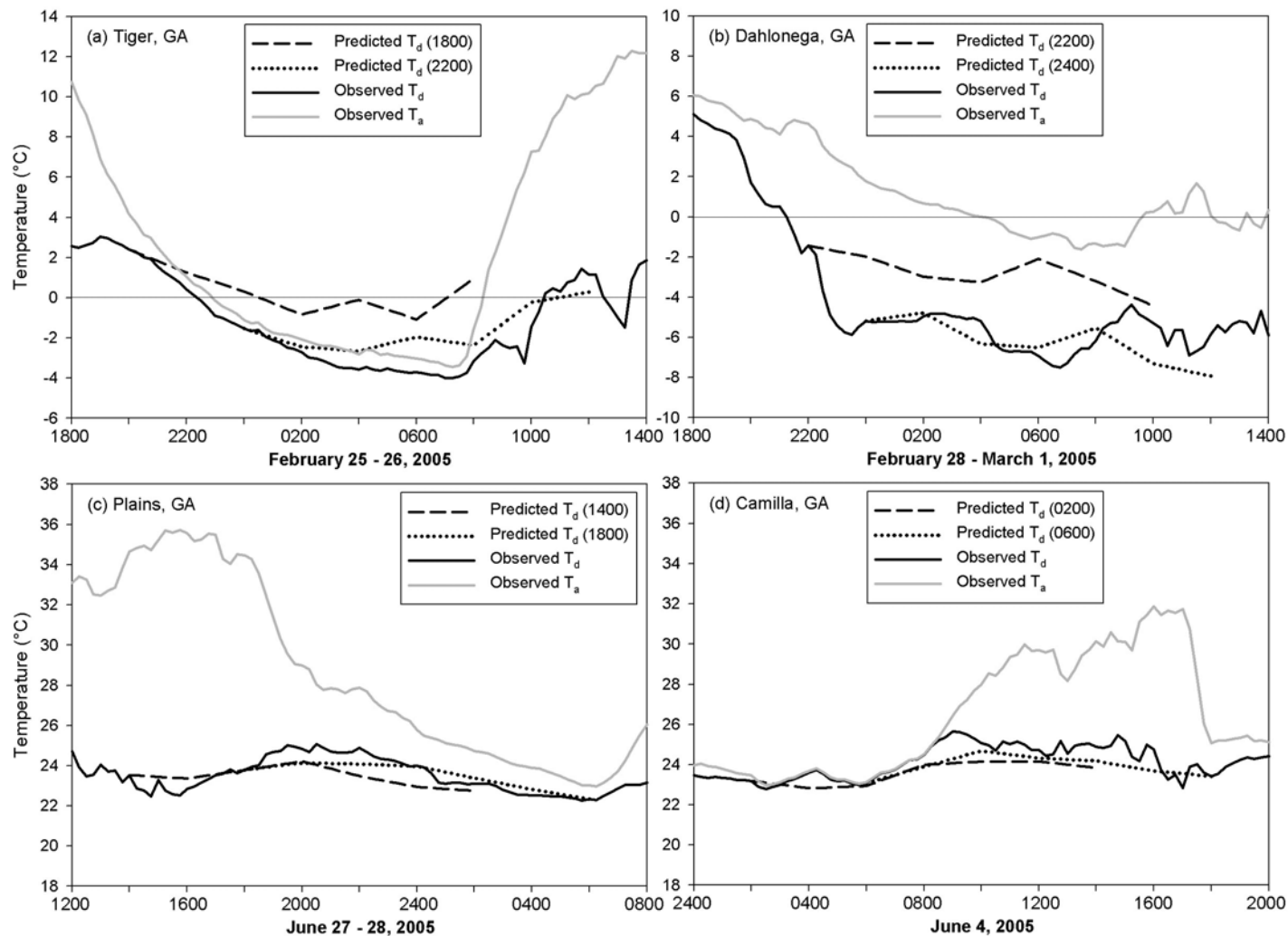
Figure 3.7: Predicted dew point temperature at two prediction times based on a sequence of twelve models for (a) Tiger, GA, (b) Dahlonega, GA, (c) Plains, GA, and (d) Camilla, GA. Observed dew point temperature and air temperature are also shown.
