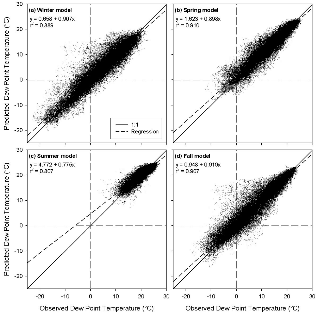
Figure 3.4: Performance of predicted dew point temperature for each seasonal model for the evaluation dataset for each corresponding season (a) winter, (b) spring, (c) summer, and (d) fall
