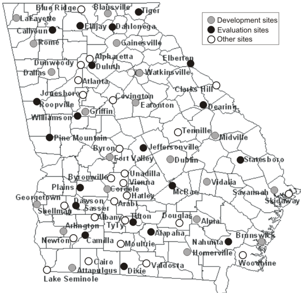
Figure 3.1: AEMN weather stations, twenty sites selected for model development and twenty sites selected for model evaluation
