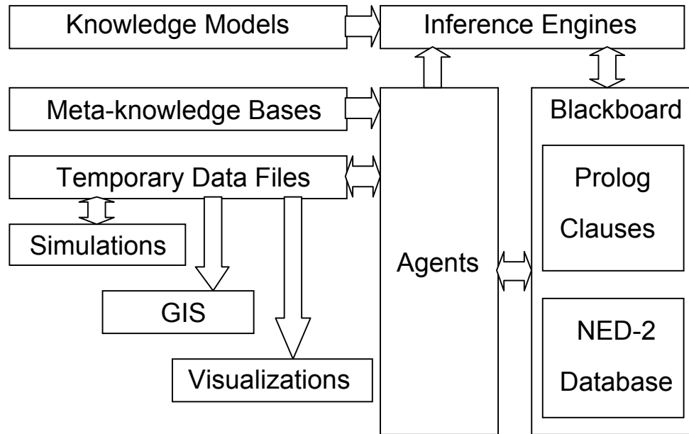
Figure 1: The NED-2 architecture
