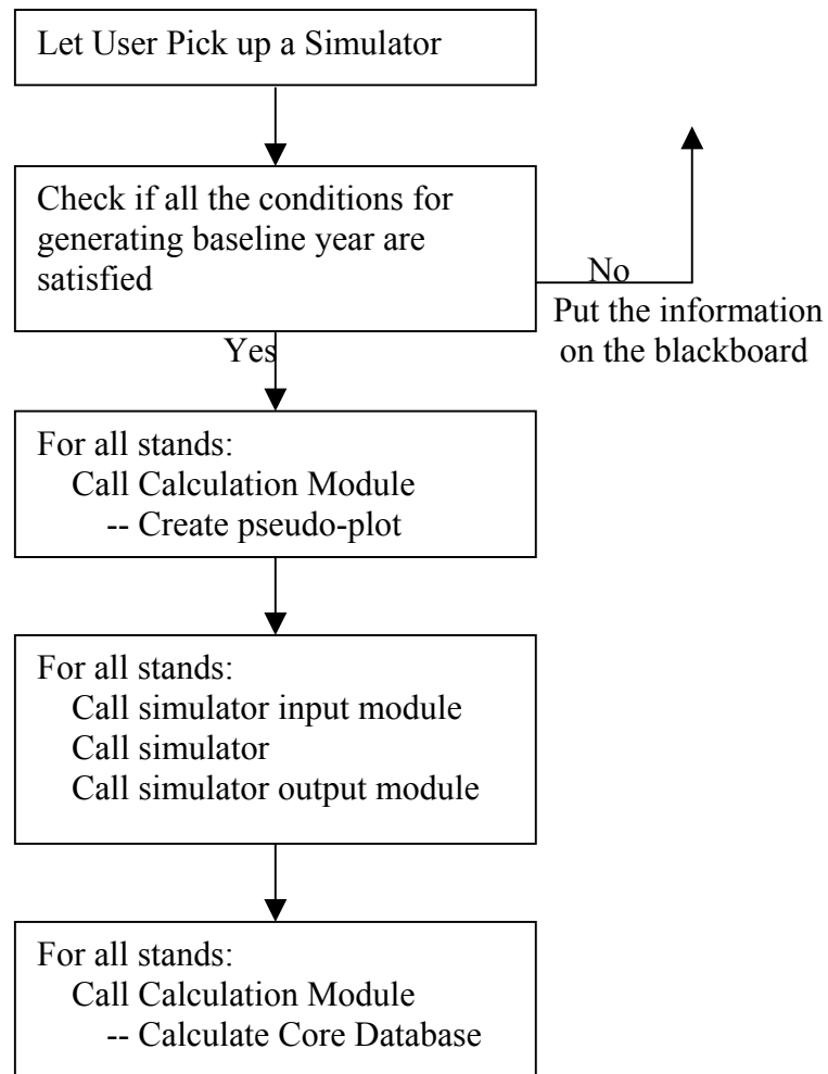
Figure 4: The procedure for baseline generation
