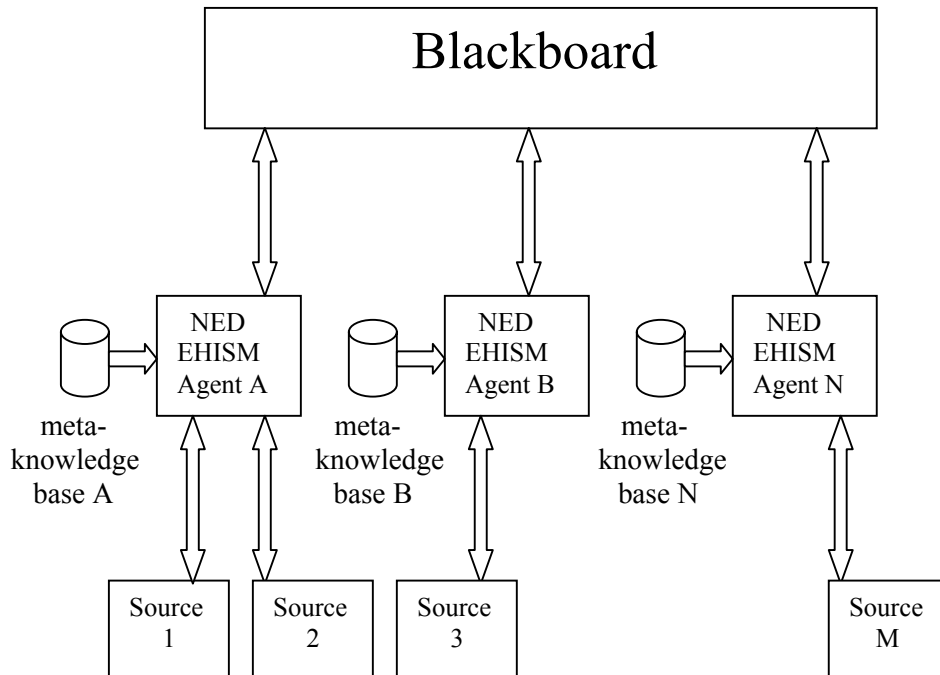
Figure 2: The NED-2 EHISM agents and their environment.
